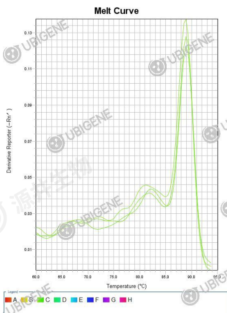
ERBB2 Stable Expression Cell Line (SK-BR-3)+hERBB2-3 melt curve
