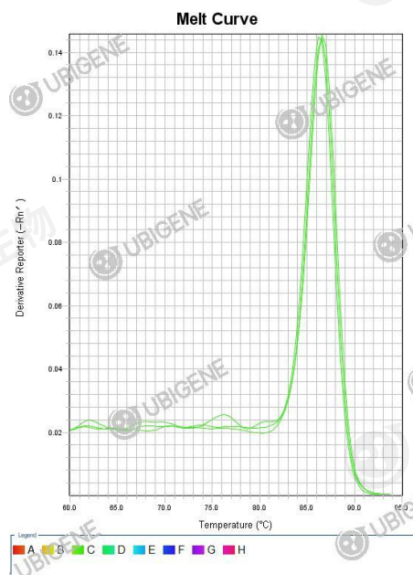
SK-BR-3_Ctrl(Puro)+β-h_actin melt curve
