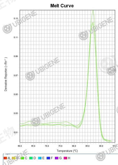
ERBB2 Stable Expression Cell Line (SK-BR-3)+β-h_actin melt curve
